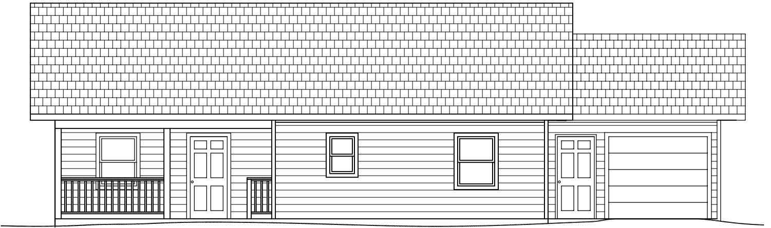
○ EAST(FRONT) ELEVATION 1/8" = 1'-0" 0 2' 4' 8'
