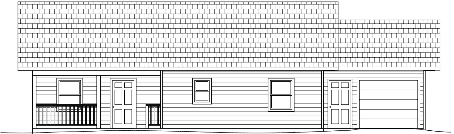
○ EAST (FRONT) ELEVATION 1/8" = 1'-0" 0 2' 4' 8'
